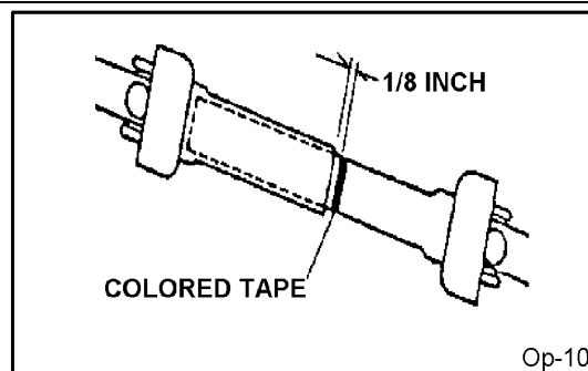
Driveline in maximum compressed position
