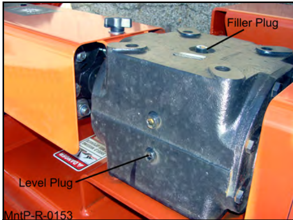
Center Gearbox
