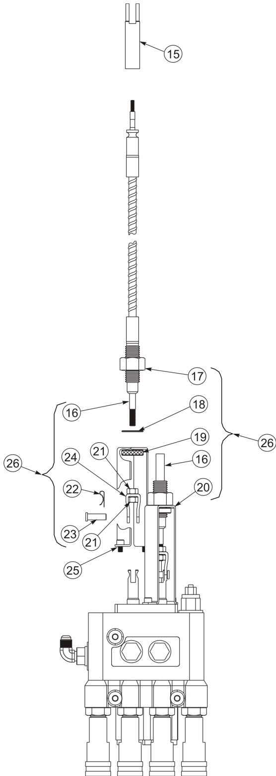
Figure 2 Cable Harness
